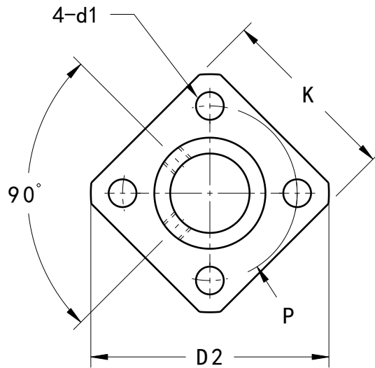
Front view Scale: 3:2
