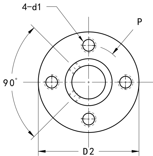
Front view[3] Scale: 3:2
