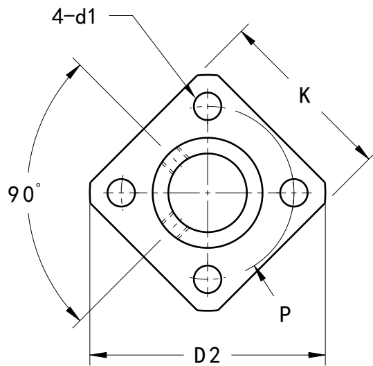
Front view Scale: 3:2
