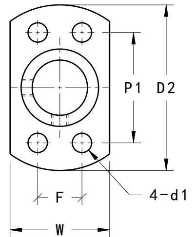
Front view Scale: 3:2
